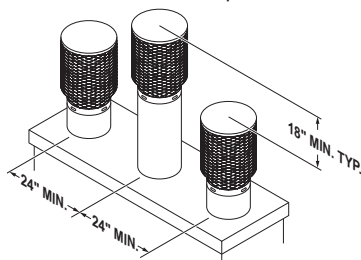
Figure 18 - Multiple Chase Installation
