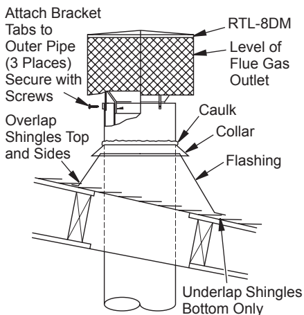
Figure 17 - Termination
