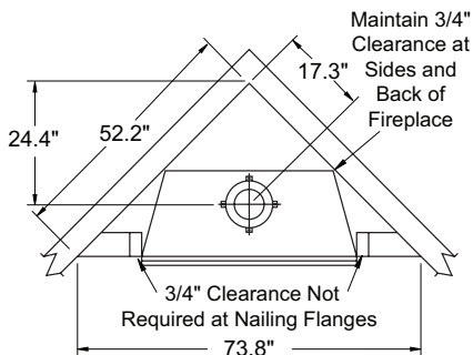
Figure 2 - Corner Installation
