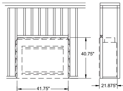
Figure 1 - Framing Dimensions
