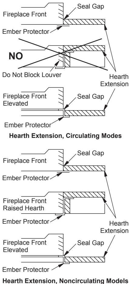
Figure 3 - Hearth Extension
