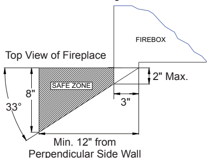
Figure 6 - Side Mantel Clearance
