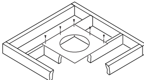
Figure 14 - Firestop Spacer with Attic Space Above Ceiling
