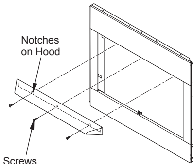
Figure 7 - Installing Hood
