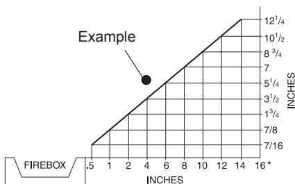
*Minimum 16" from Side Wall Figure 2 - Minimum Clearance for Combustible to Wall
