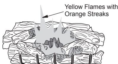
Figure 23 - Correct Burner Flame Pattern
