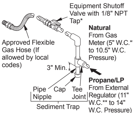
Figure 13 - Gas Connection
