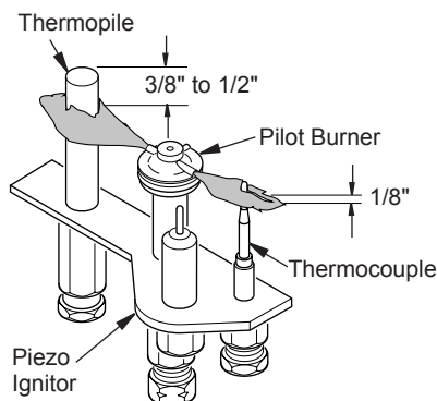
Figure 22 - Pilot Assembly
